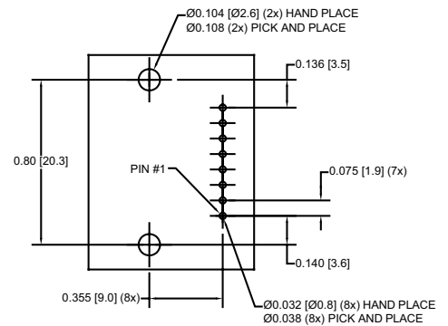
COMPONENT SIDE
